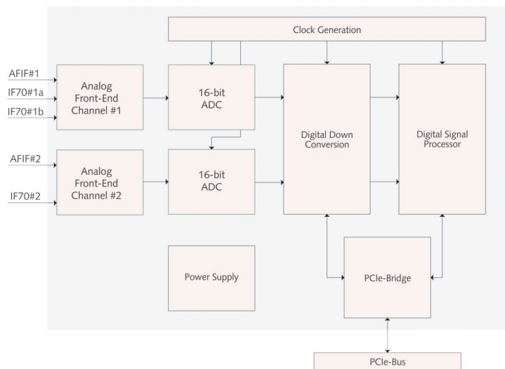
W-PCIe block diagram
